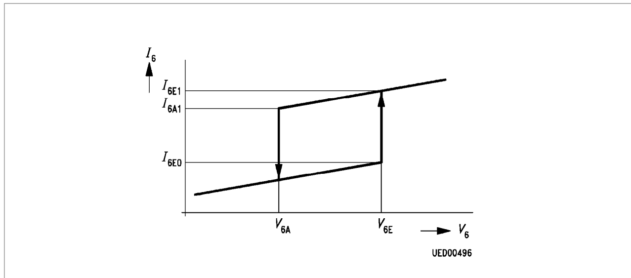
Start-Up Hysteresis
